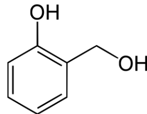
Salicyl alcohol
