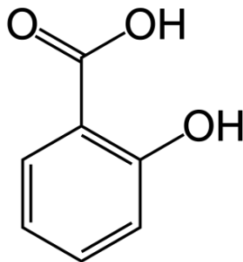
Salicylic acid
